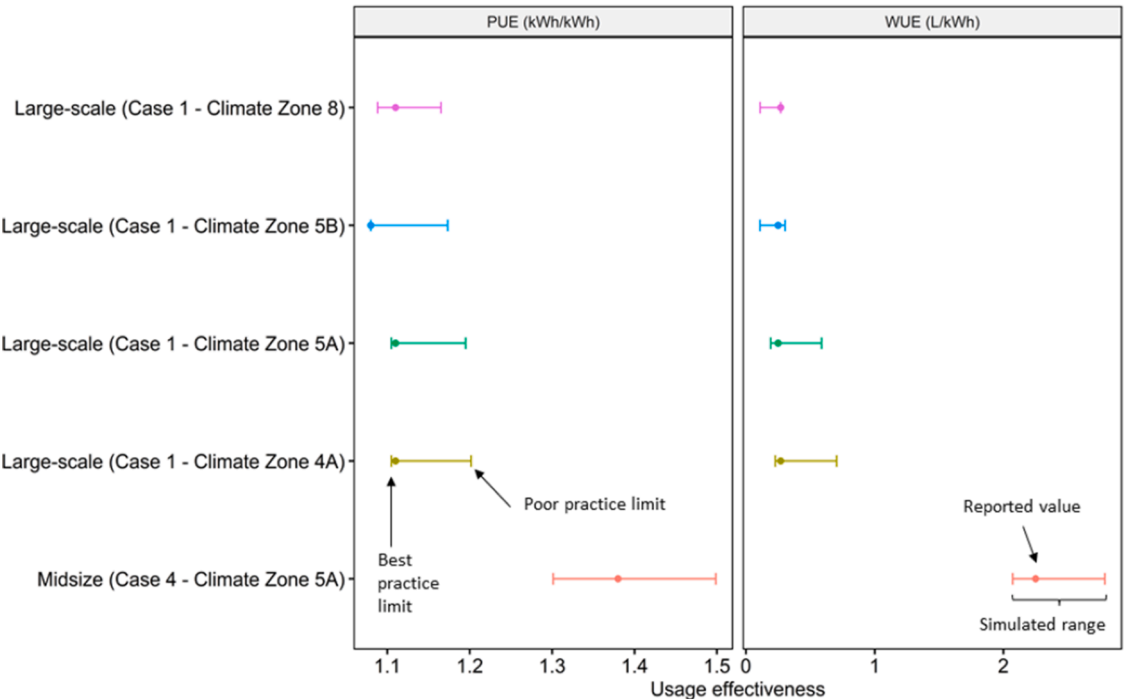
Fig. 4. Simulated PUE and WUE ranges versus reported values.
