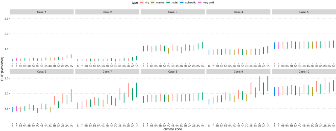
Fig. 5. Annual average PUE simulation results for 10 DC cases and 15 U.S. climate zones.
