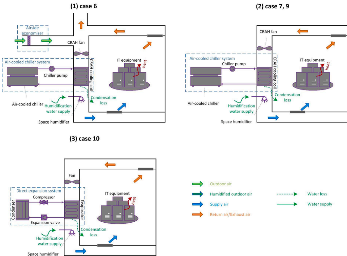
Fig. 2. Schematic diagrams of considered DC space conditioning system configurations (CRAH = computer room air handler).
